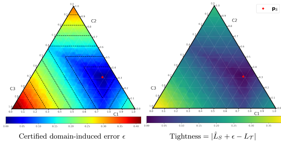
Fig. 2: The certified error (left) and its tightness (right), according to the variant \|\mathbf{d}_+\|_{\infty} \cdot \|\ell_h\|_1 on the satimage data set, using a logistic regression and the zero-one loss.
