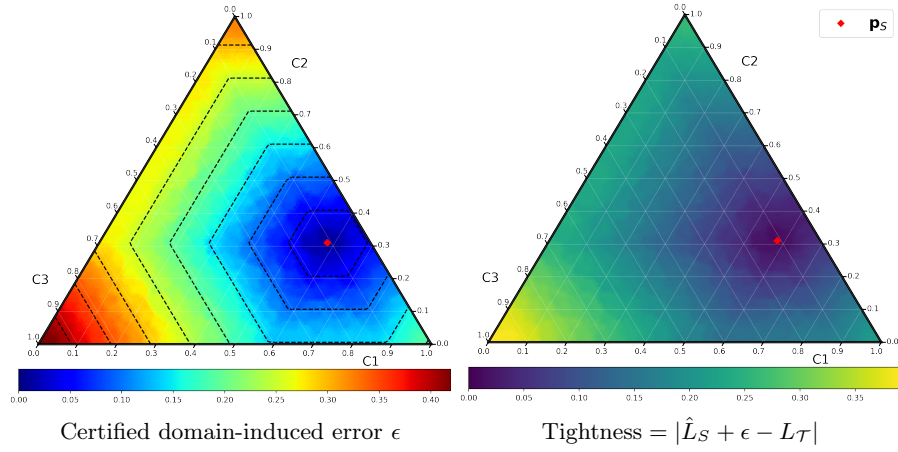
Fig. 1: The certified error (left) and its tightness (right), according to \|\mathbf{d}\|_{\infty} \cdot \|\ell_h\|_1 on the satimage data set, using a logistic regression and the zero-one loss.
